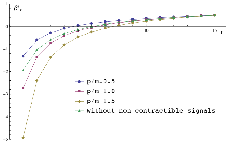
Figure 2: The equilibrium contractual incentives: N = 15 , \gamma = 0.95 , \frac{b}{m} = 0.5 , v_\varepsilon^2 = v_\nu^2 = v_\theta^2 .
