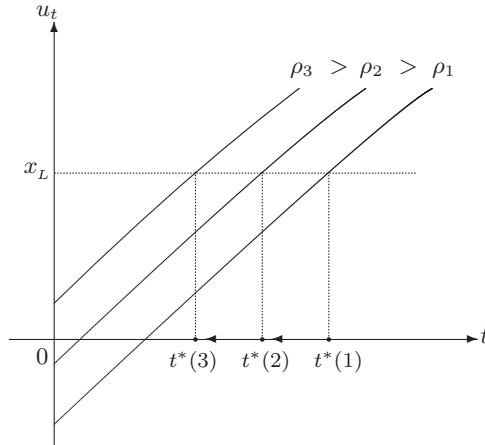
Figure 5.1: u_t in t \geq 0 for three different values of \rho .
