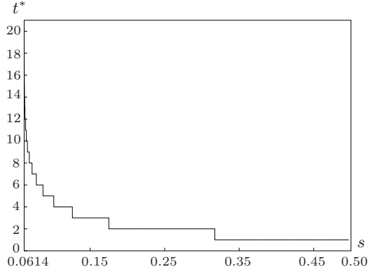
(I): Monotonicity of t^* in s
