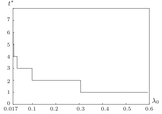
(II): Monotonicity of t^* in \lambda_0
