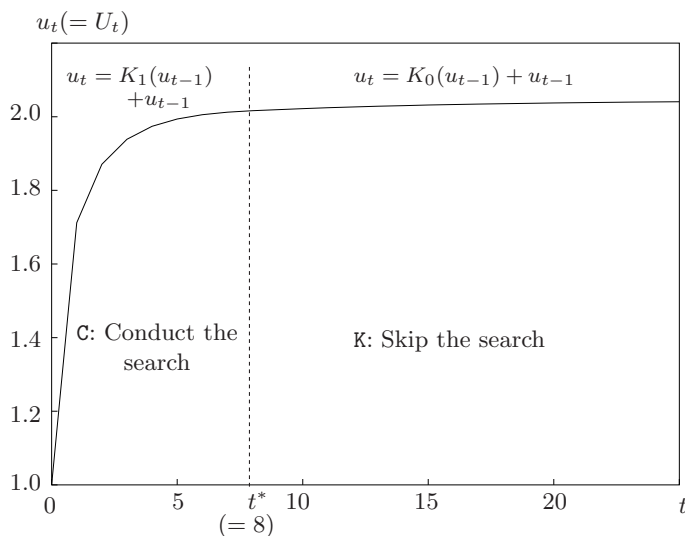
Figure 7.2: Time threshold t^* for conducting search
