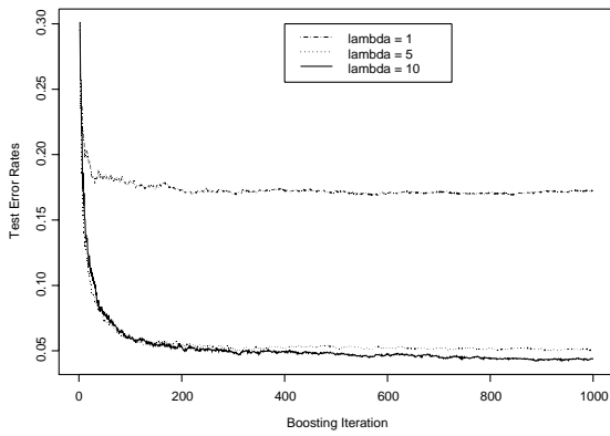
(c) MarginBoost. L_1
