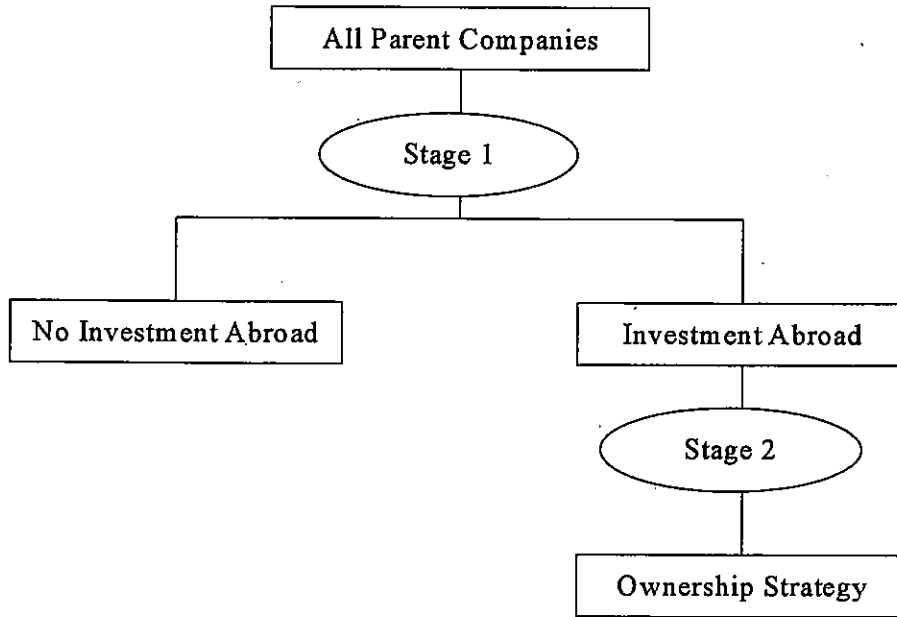
Figure 1: Model Structure
